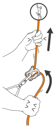
4.1 FEEDING
