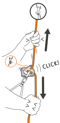
4.2 LOCKING TEST
