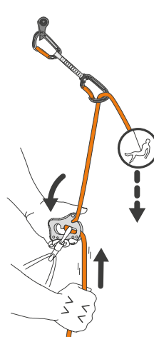
5.4 LOWERING
